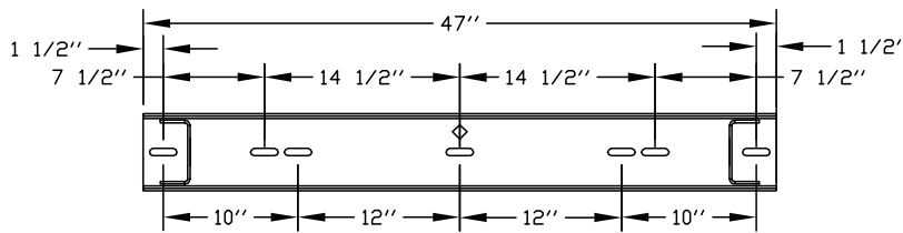
RAIL BRACKETS
