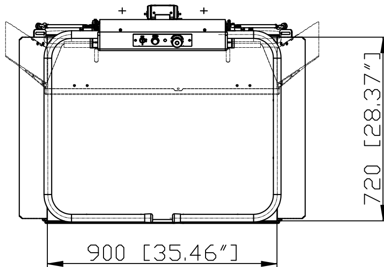
PLF_OMEGA (720X900) STRAIGHT ENTRANCE
