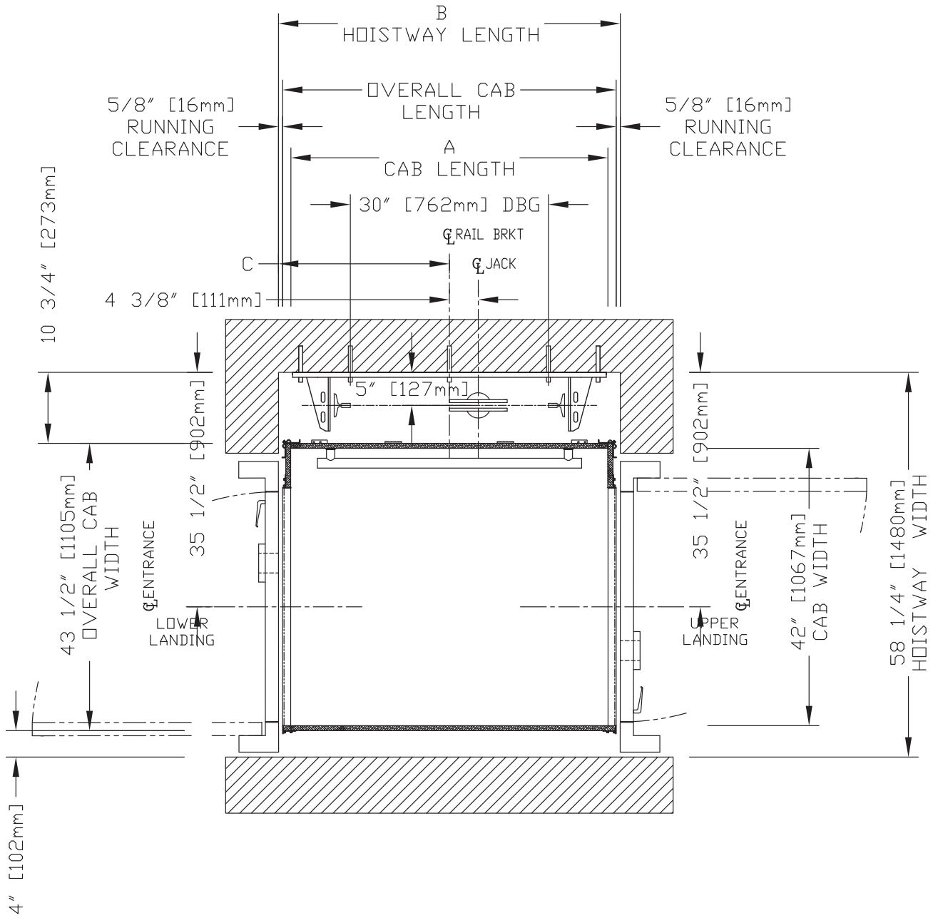
HOISTWAY DIMENSIONS
