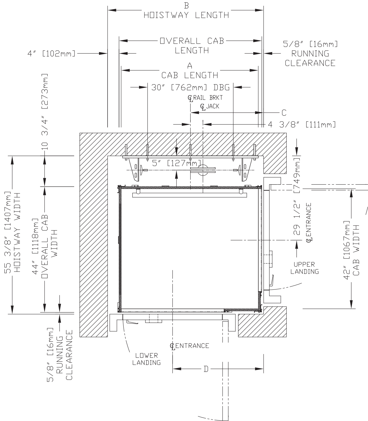
HOISTWAY DIMENSIONS
